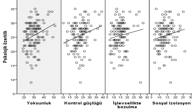
Model Summary b
